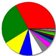
Coal, 18 MJ per kg, in ground; Coal, 29.3 MJ per kg, in ground; Coal, brown, 8 MJ per kg, in ground; Uranium, 360 MJ per kg, in ground; Coal, natural, 20 MJ per MJ, in ground; Coal, brown, in ground; Energy from gas, natural; Coal, natural, 20 MJ per MJ, in ground; Coal, hard, unspecified, in ground; Gas, mine, off-gas, process, coal refining; Uranium ore, 1.1 MJ per kg, in ground; Processo remanente; Coal, natural, in ground; Coal, natural, 20 MJ per MJ, in ground; Gas, mine, off-gas, process, coal refining; Coal, 20 MJ per kg, in ground
