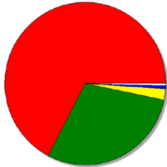
Methane, bromochlorodifluoro-, Halon 1211; Methane, bromotrifluoro-, Halon 1301; Methane, chlorodifluoro-, HCFC-22; Methane, tetrachloro-, CFC-10; Methane, trichlorofluoro-, CFC-11; Processo remanente
